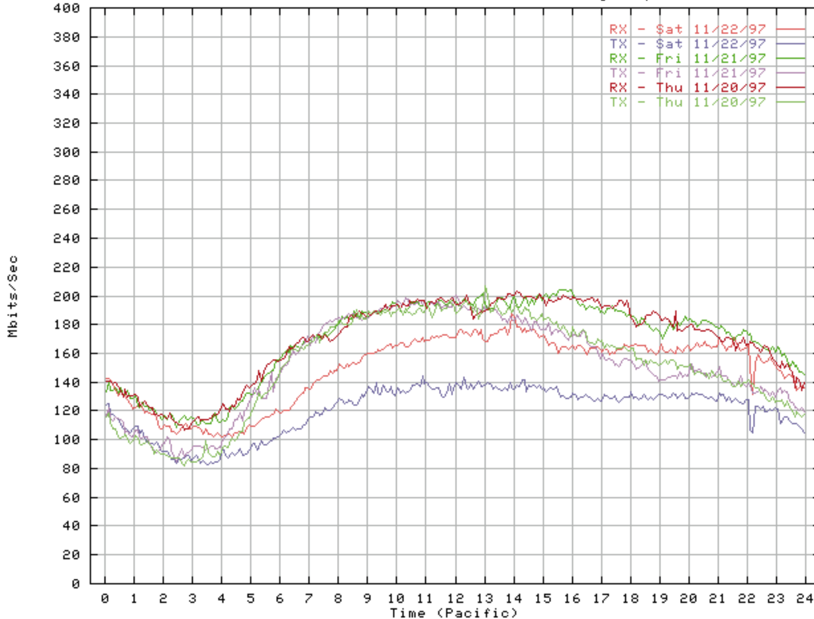
MAE West - Links to Ames (4 x OC3c) - 3 day composite
