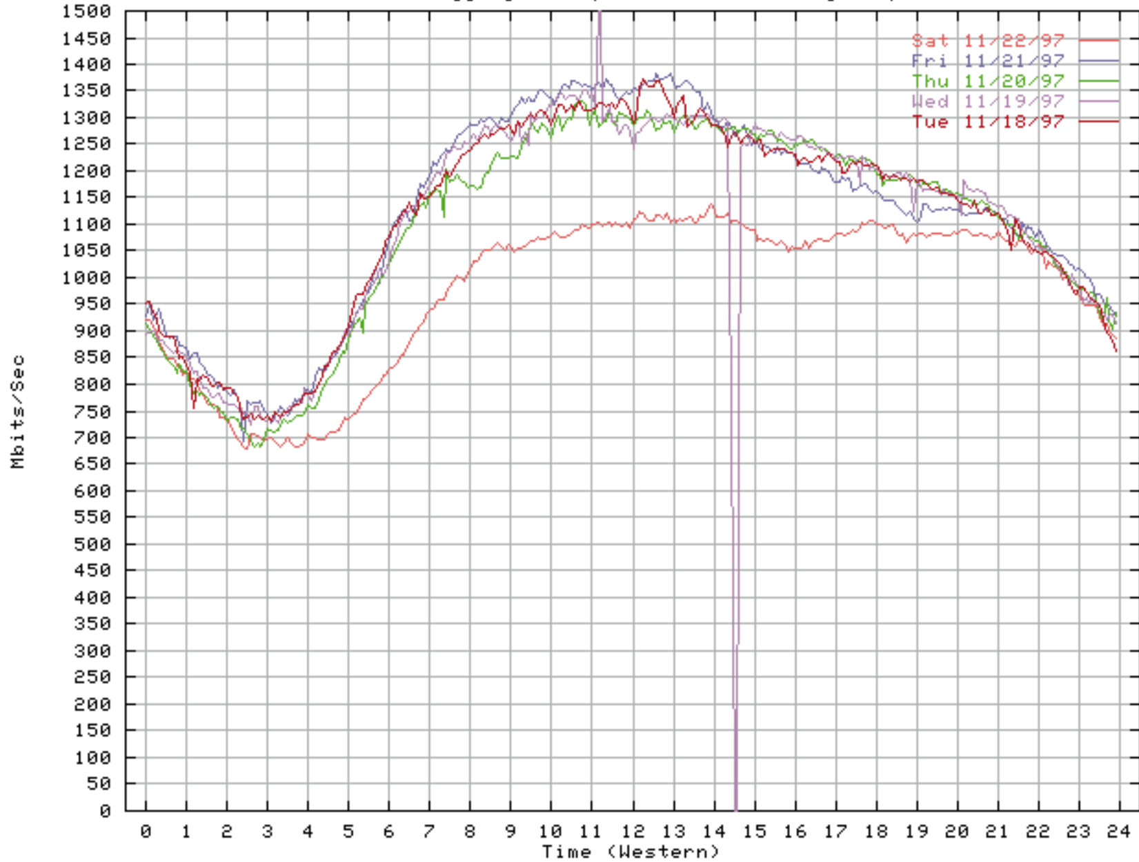
MAE West - Aggregate Input Traffic - 5 day composite
